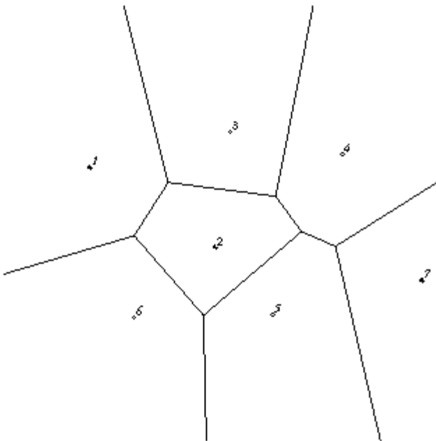
Figure 14-3 : Dirichlet Domains
