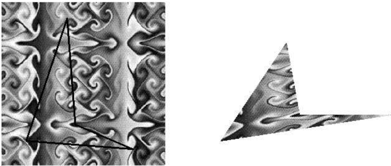
Figure 9-1 : Texture-Mapping Process
