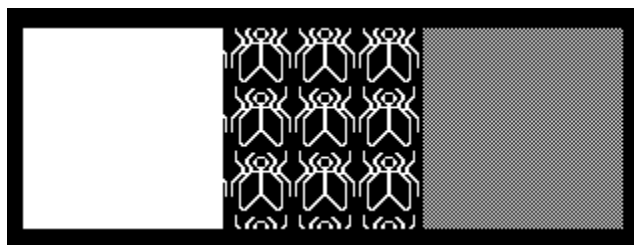
Figure 2-11 : Stippled Polygons
