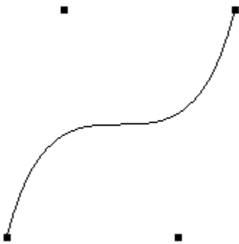
Figure 12-1 : Bezier Curve
