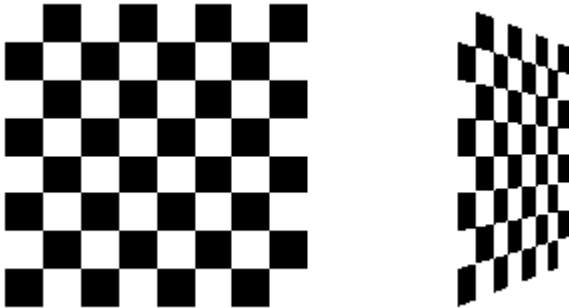
Figure 9-2 : Texture-Mapped Squares
