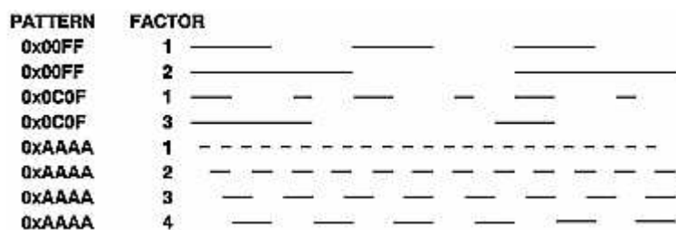
Figure 2-8 : Stippled Lines
