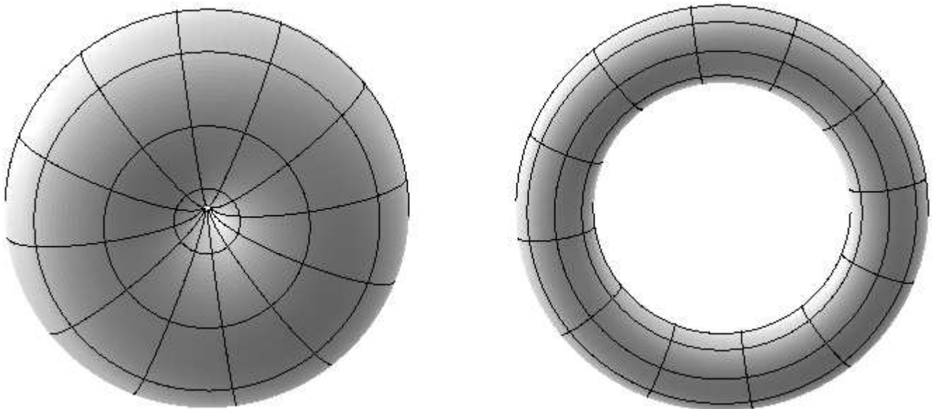
Figure 9-6 : Texture-Map Distortion
