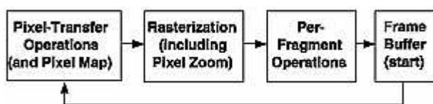
Figure 8-5 : glCopyPixels() Pixel Path
