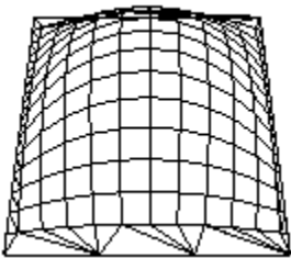
Figure 12-4 : NURBS Surface
