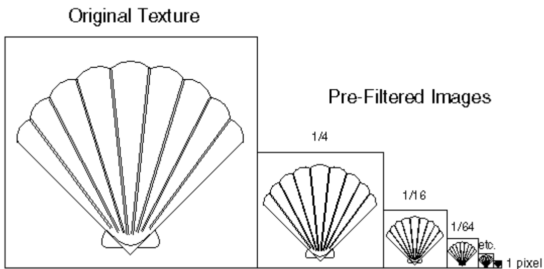
Figure 9-4 : Mipmaps
