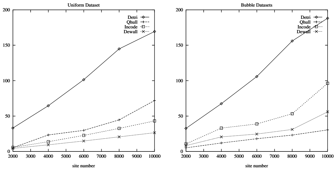
Figure 9: The algorithm times in seconds: uniform datasets on the left, bubble on the right.
